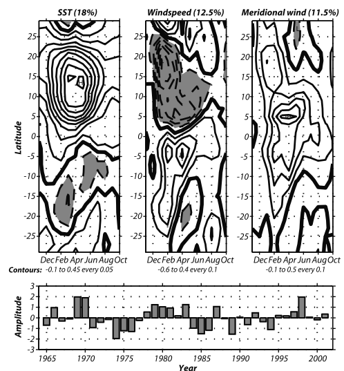
Figure 2. Leading EOF of combined tropical Atlantic SST ( ^{\circ}\text{C} ), windspeed and meridional wind (both in \text{m s}^{-1} ), averaged across the width of the basin and arranged in yearly samples of latitude-by-calendar month. Data are from November 1964 to October 2001. Negative contours dashed and shaded. The contour intervals are indicated below each panel. Percent variance explained in each field is shown in parentheses above. The time series corresponding to the combined EOF is shown below, one value for each year of the corresponding January.
